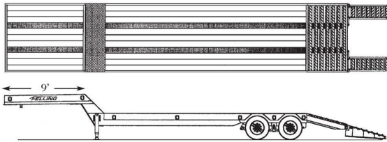
Shown with Optional 45° 9' Upper Deck
