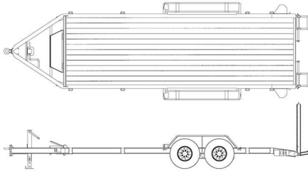
Shown with optional Toolbox & 2' Dovetail.
